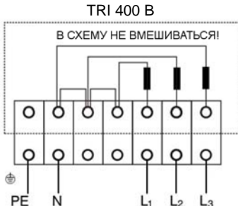
ECOSUN S+ 30 - 36
